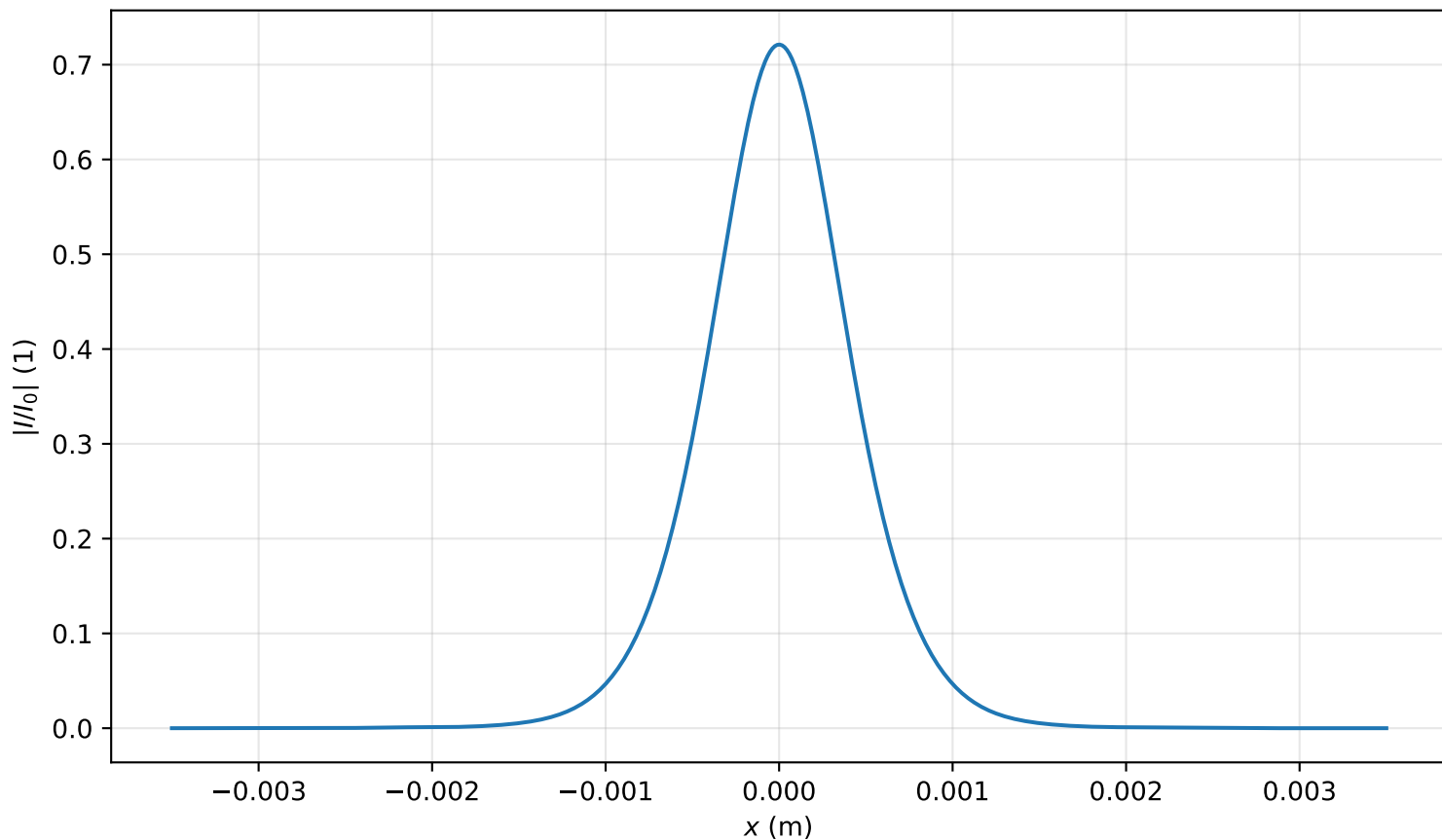
Intensity profile I(x, y = 0, z = 3.503m)/I_0 , P_{in}=0.7P_{cr} , artificial time
